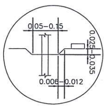
CONTRACTION JOINT 1 : 25
